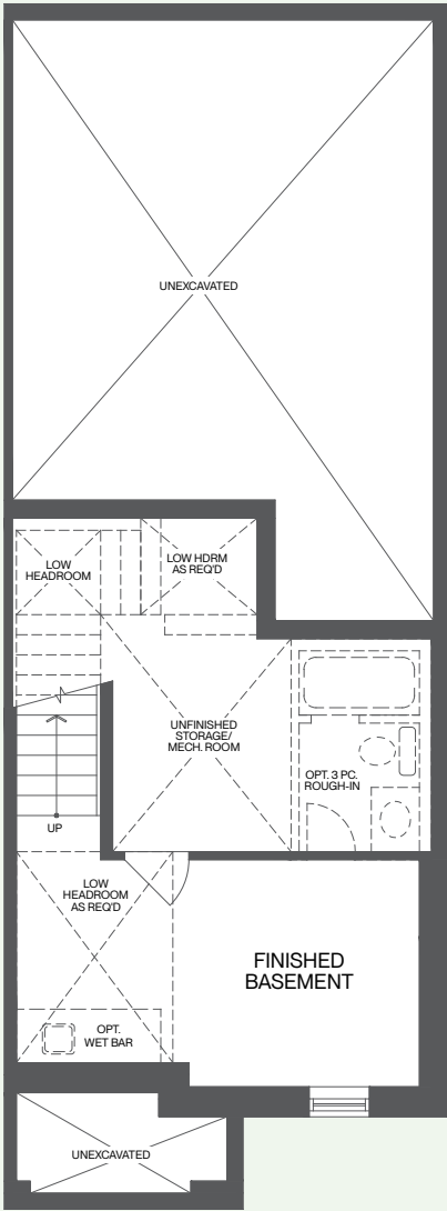
Basement Plan, El. 'A & B'
